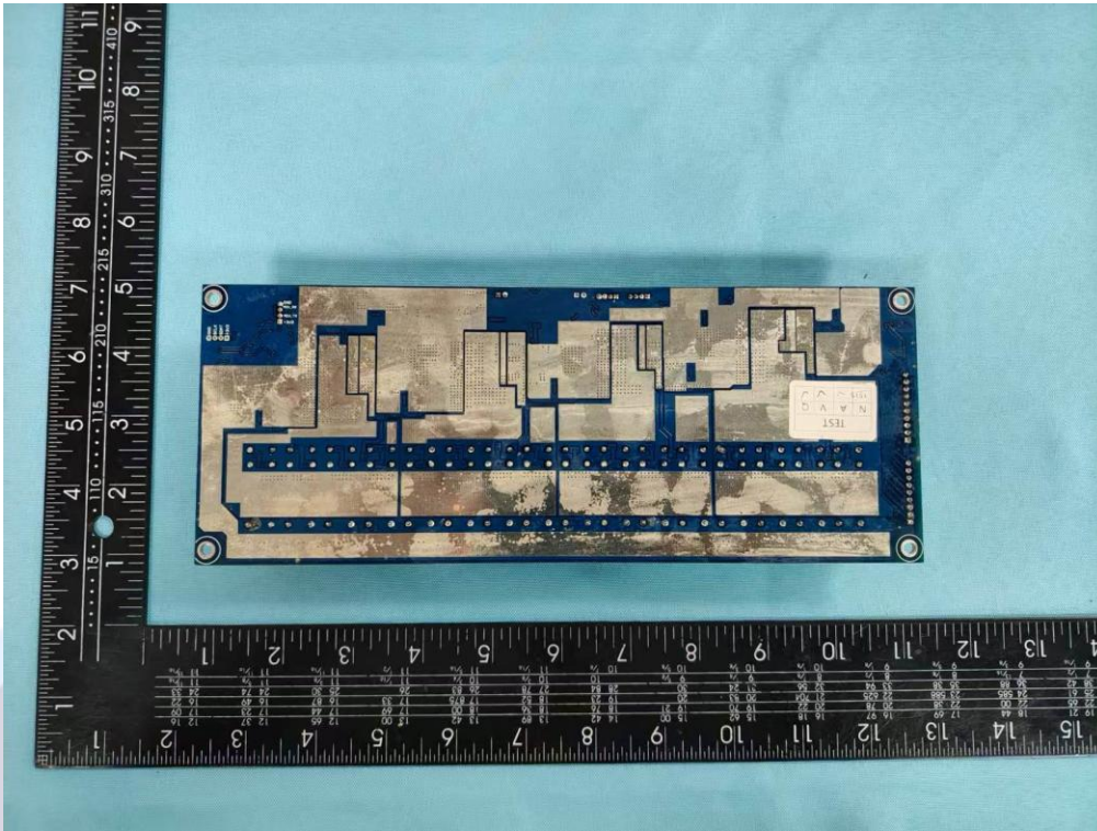
Picture 5. Front view of PCB
