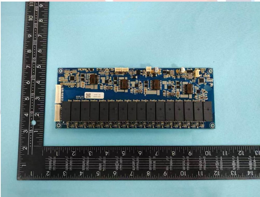
Picture 6. Back view of PCB
